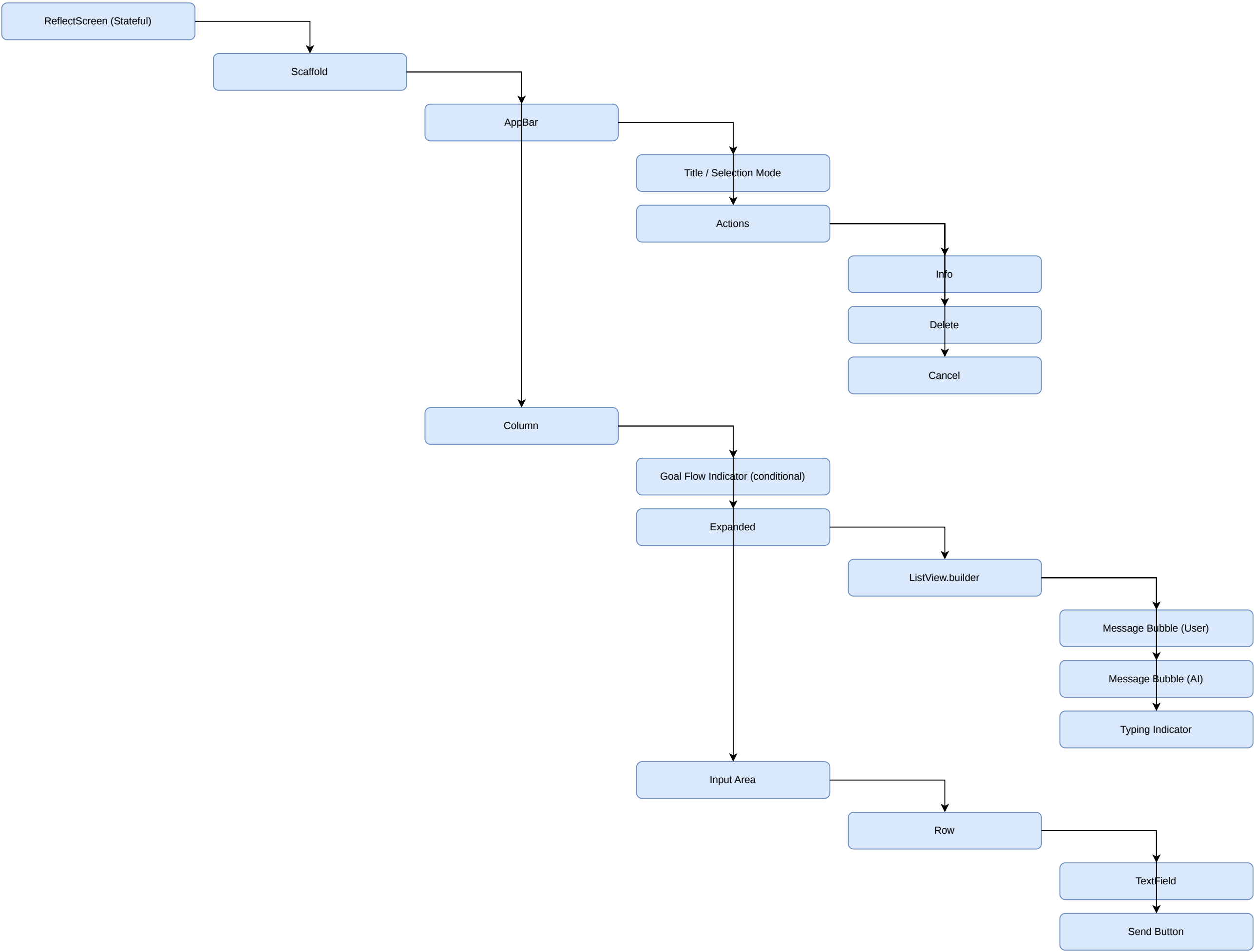
WIDGET TREE — 6. Reflect Chat
