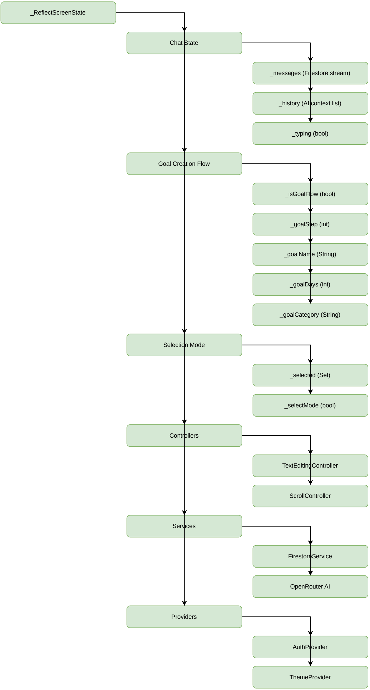
STATE TREE — 6. Reflect Chat
